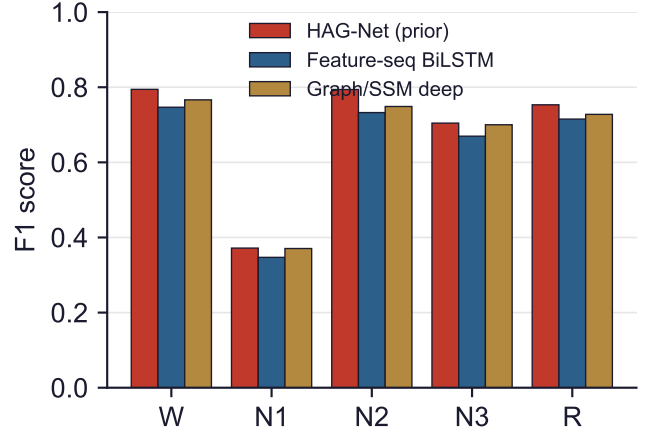
Fig. 2. Per-stage F1. N2/N3/Wake are scored reliably; N1 is hardest. Event features and the EOG/EMG channels improve REM and N1.
