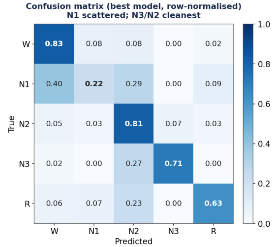
Fig. 3. Confusion matrix (row-normalized). Most error is N1 mislabelled as Wake, N2 or REM, the known ambiguity of transitional sleep.
