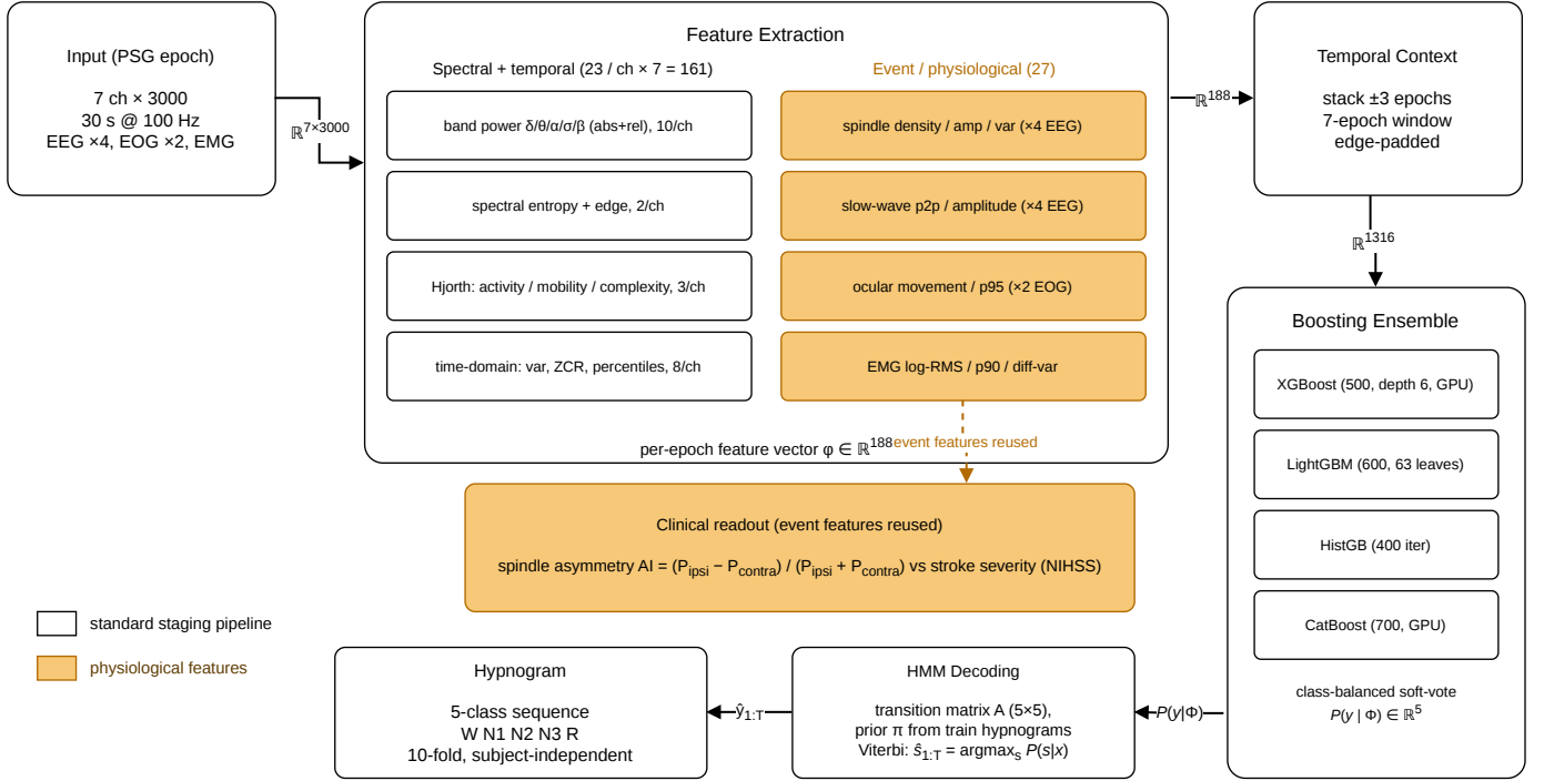
Fig. 1. HAG-Net pipeline (physiological components highlighted). An overnight seven-channel PSG is harmonized, epoched, and mapped to a dual spectral/event feature representation ( \phi \in \mathbb{R}^{188} ); a \pm 3 -epoch temporal-context window feeds a class-balanced gradient-boosting classical prior whose per-epoch posteriors are refined by hidden-Markov Viterbi decoding into the five-class hypnogram. The hemispheric-asymmetry graph module and the bidirectional selective state-space decoder (detailed in Section IV-D, eqs. (6)–(9)) supply a residual, tanh-gated correction to the prior; on this cohort that correction is rejected on validation, so the realized staging path is the prior+HMM shown here. Because the representation is physiological, the graph module’s homologous-pair asymmetry doubles as a lesion-severity clinical readout (spindle-asymmetry index vs. NIHSS), and a split-conformal layer emits calibrated prediction sets.
