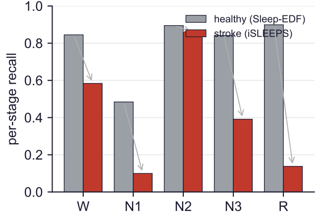
Fig. 5. Zero-shot healthy→stroke transfer. Accuracy falls -0.27 , concentrated in REM and N3; N2 is comparatively robust.
